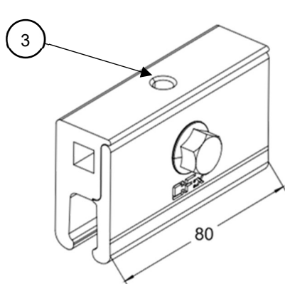
RD80-Clamp
